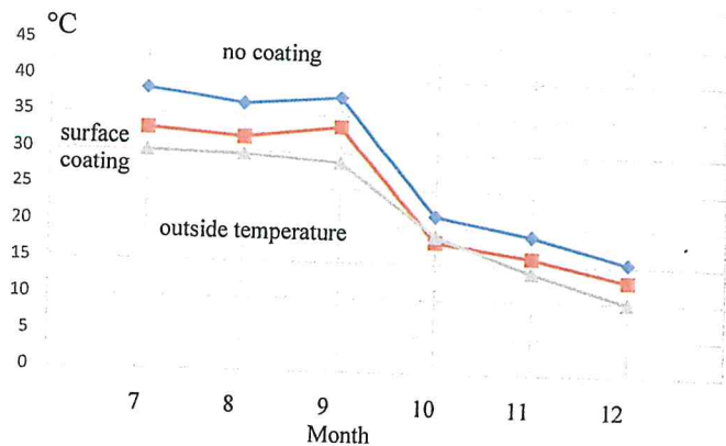
Figure 3: The change of room air temperature.
