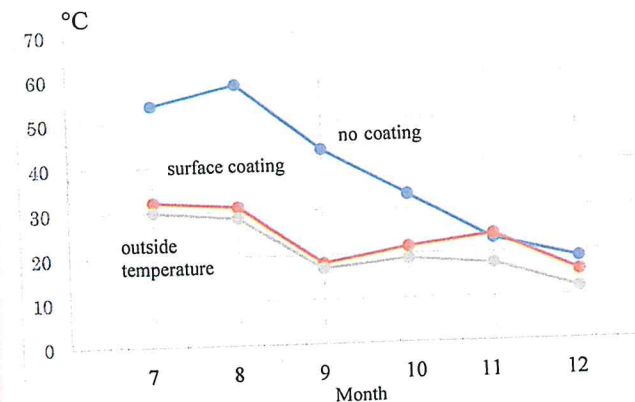
Figure 2: The change of roof surface temperature after applying Adgreencoat.
